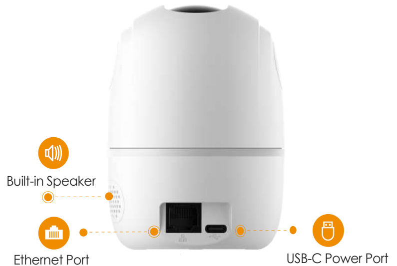
Back View
